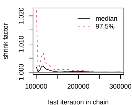
d.III.III_Amivantamab
